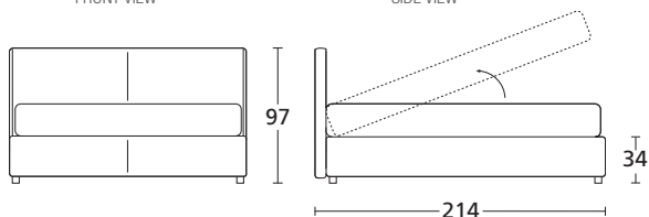
VISTA FRONTALE FRONT VIEW
