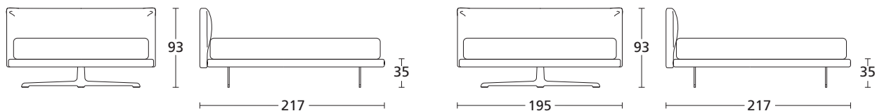
VISTA FRONTALE FRONT VIEW
